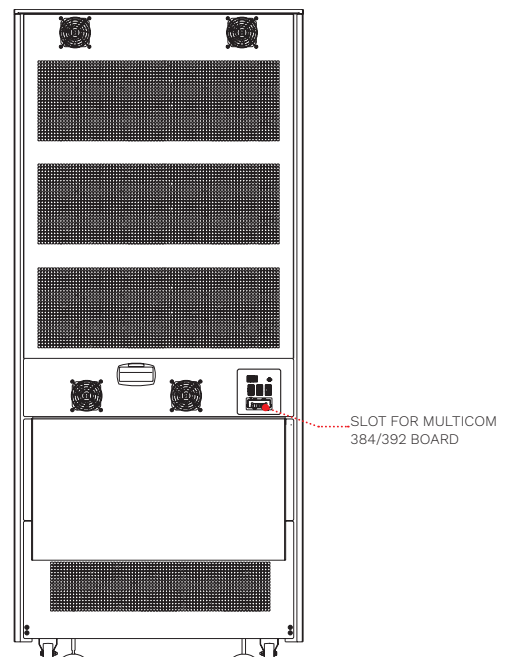
MST 160-200 (rear)
