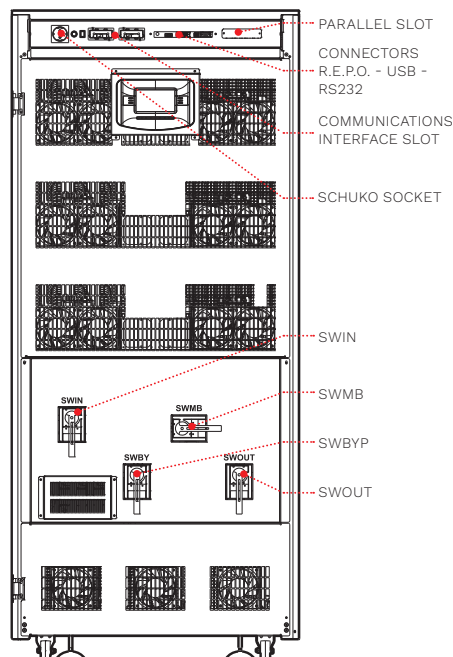
MST 160-200 (front)
